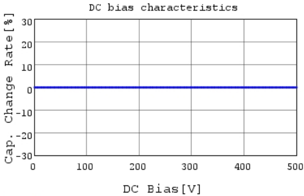
GQM22M5C2H120JB01 C-DC bias capchange, 25.0c
