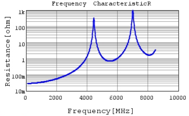
GQM22M5C2H120JB01 R DC0V, 25degC
