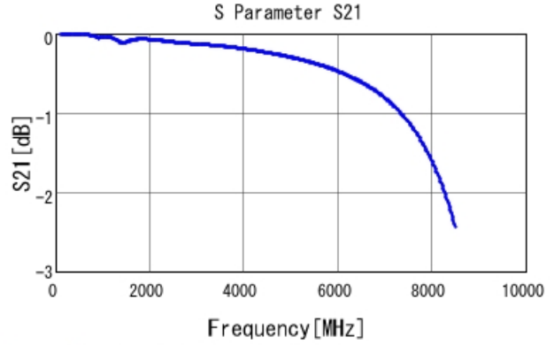
GRM1885C1H301GA01 S21 DCOV, 25degC
