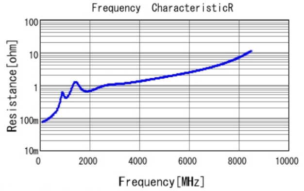
GRM1885C1H301GA01 R DCOV, 25degC
