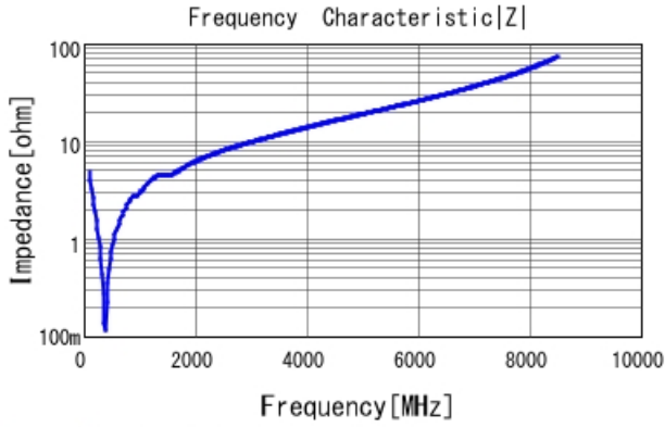
GRM1885C1H301GA01 |Z| DCOV, 25degC
