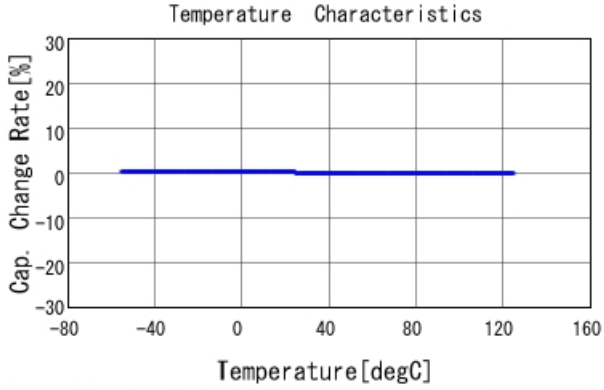
GRM1885C1H301GA01 C-Temp. capchange, DCOV, AC1Vrms
