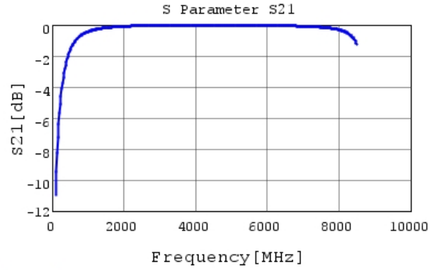
GQM1555C2D4R7CB01 S21 DCOV, 25degC
