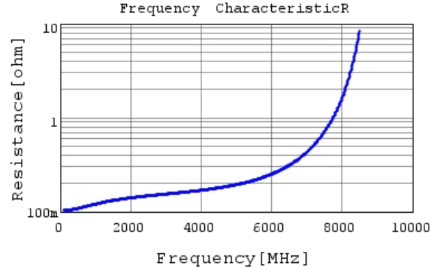
GQM1555C2D4R7CB01 R DC0V, 25degC
