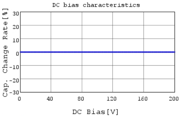
GQM1555C2D4R7CB01 C-DC bias capchange, 25.0c
