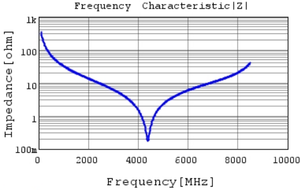
GQM1555C2D4R7CB01 |Z| DC0V, 25degC
