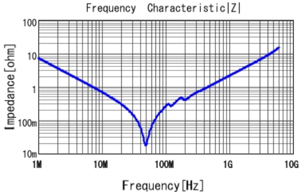
GRM2165C1H223JA01 |Z| DCOV, 25degC
