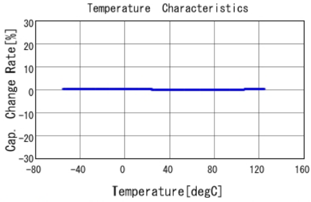
GRM2165C1H223JA01 C-Temp. capchange, DCOV, AC1Vrms
