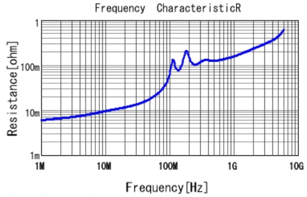
GRM2165C1H223JA01 R DCOV, 25degC
