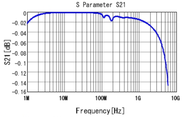
GRM2165C1H223JA01 S21 DCOV, 25degC
