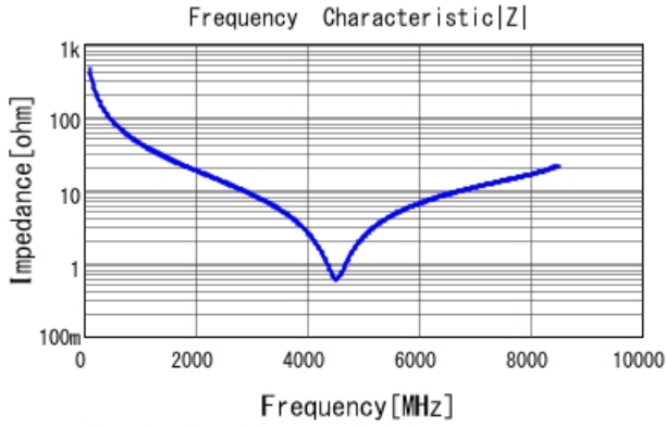
GRM1555C1H3R5CA01 |Z| DCOV, 25degC
