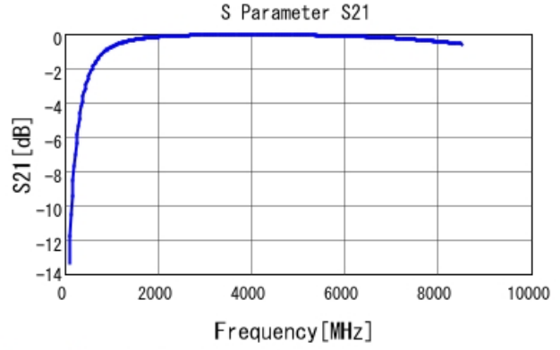
GRM1555C1H3R5CA01 S21 DC0V, 25degC
