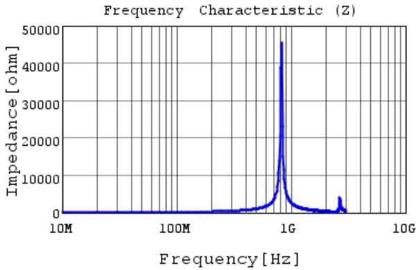
LQW2UASR22G0C |Z|
