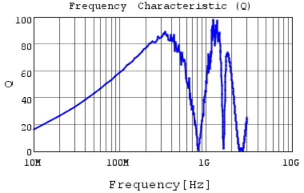
LQW2UASR22G0C Q
