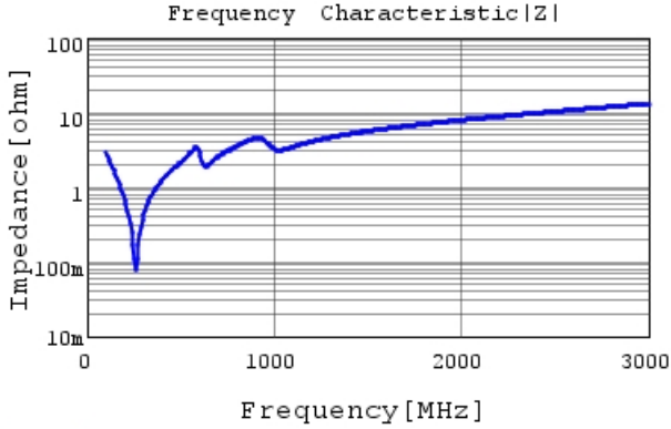
GRM31A5C3A471JWA1 |Z| DC0V, 25degC
