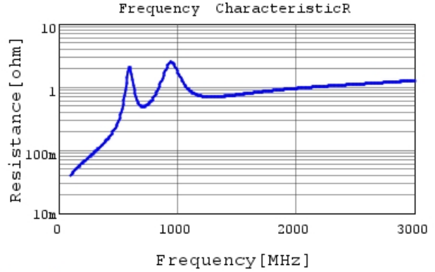
GRM31A5C3A471JWA1 R DC0V, 25degC
