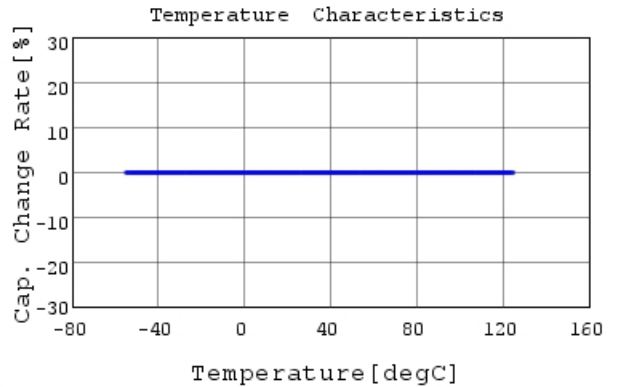
GRM31A5C3A471JWA1 C-Temp. capchange, DC0V, 1
