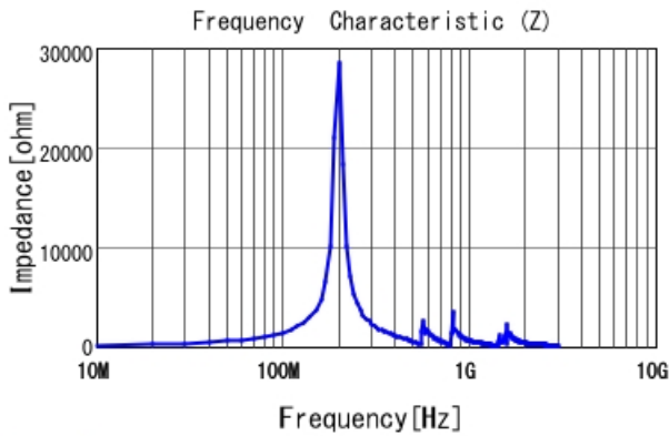
LQW2UAS1R8J0C |Z|
