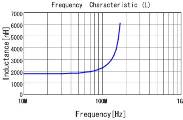
LQW2UAS1R8J0C L
