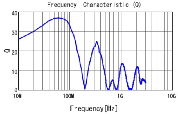
LQW2UAS1R8J0C Q
