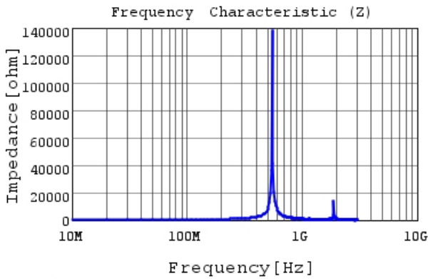
LQW2UASR47F0C |Z|
