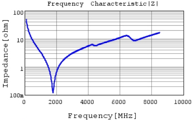
GJM0335C1E330JB01 |Z| DCOV, 25degC
