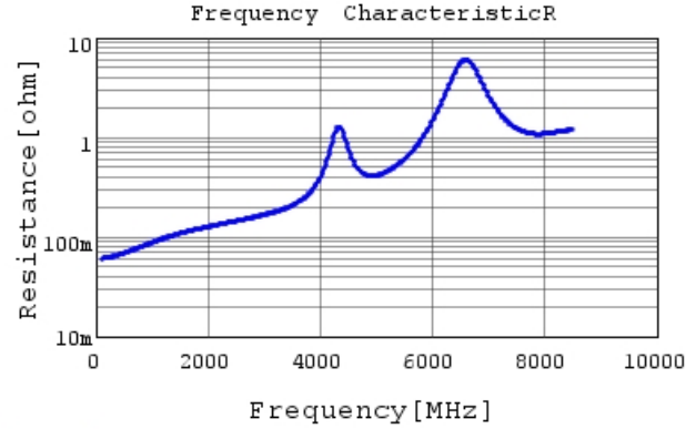
GJM0335C1E330JB01 R DCOV, 25degC
