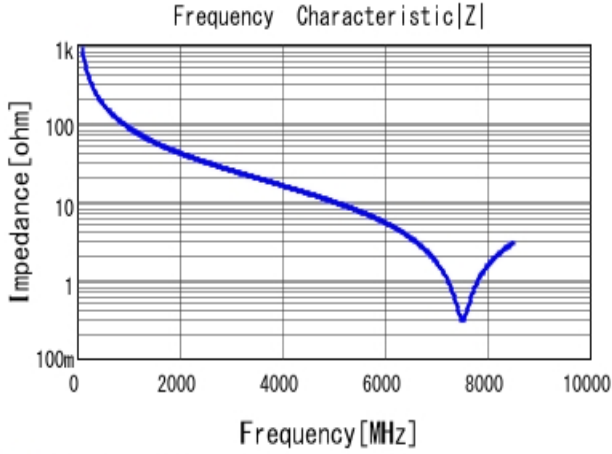
GJM0335C1E1R8BB01 |Z| DC0V, 25degC
