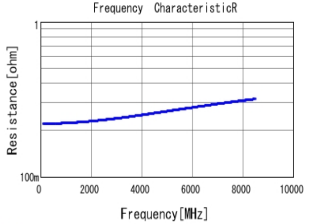
GJM0335C1E1R8BB01 R DC0V, 25degC
