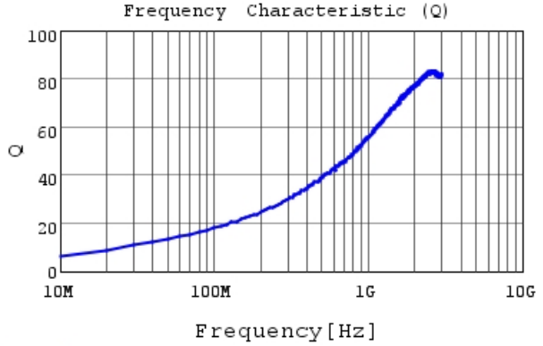
LQG15WZ3N3C02 Q
