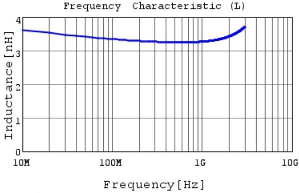
LQG15WZ3N3C02 L
