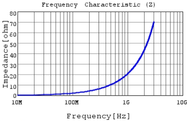
LQG15WZ3N3C02 |Z|
