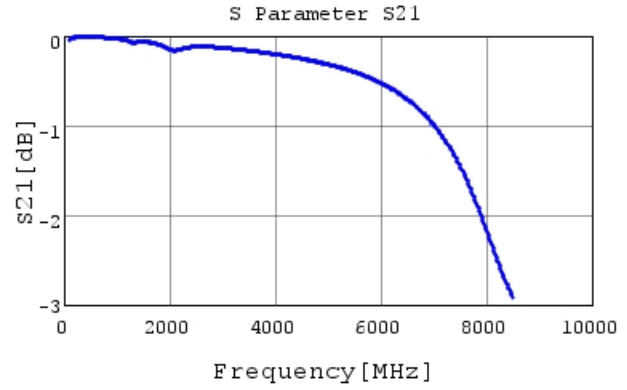
GCM1885C2A151JA16 S21 DCOV, 25degC
