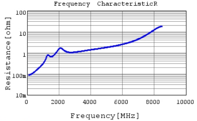
GCM1885C2A151JA16 R DC0V, 25degC
