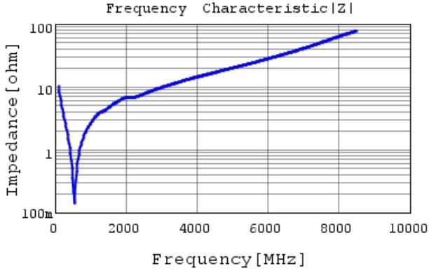
GCM1885C2A151JA16 |Z| DC0V, 25degC
