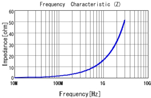
LQP03TN2N5B02 |Z|
