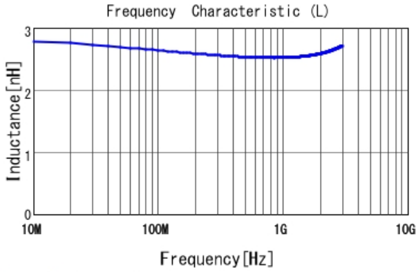
LQP03TN2N5B02 L
