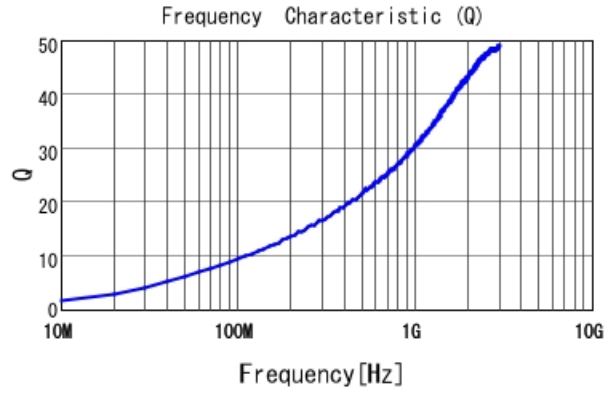
LQP03TN2N5B02 Q
