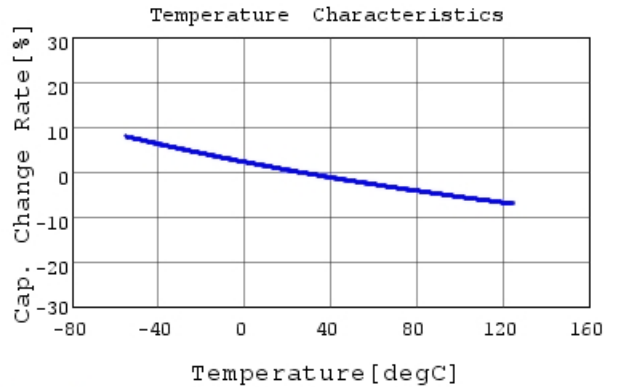
GRM31A7U3A180JW31 C-Temp. capchange, DC0V, 1
