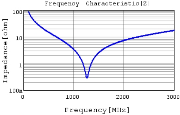
GRM31A7U3A180JW31 |Z| DC0V, 25degC
