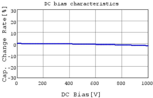
GRM31A7U3A180JW31 C-DC bias capchange, 25.0c
