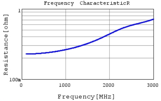
GRM31A7U3A180JW31 R DC0V, 25degC
