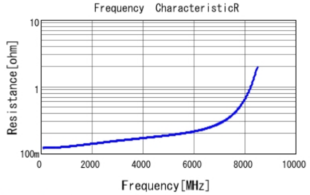
GQM1555C2D2R2BB01 R DCOV, 25degC
