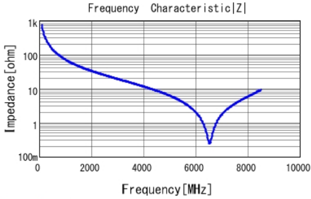
GQM1555C2D2R2BB01 |Z| DCOV, 25degC
