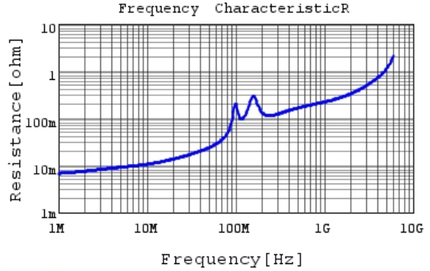
GRM3195C1H183JA01 R DCOV, 25degC
