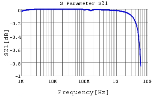
GRM3195C1H183JA01 S21 DCOV, 25degC
