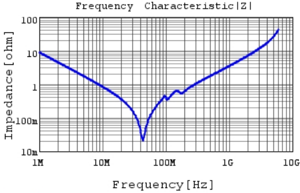
GRM3195C1H183JA01 |Z| DCOV, 25degC
