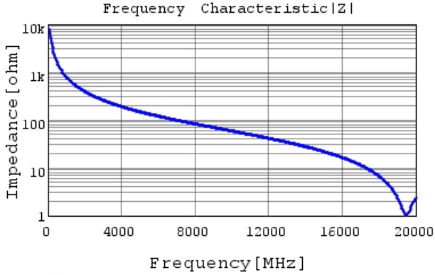
GRM0335C1HR20WA01 |Z| DCOV, 25degC
