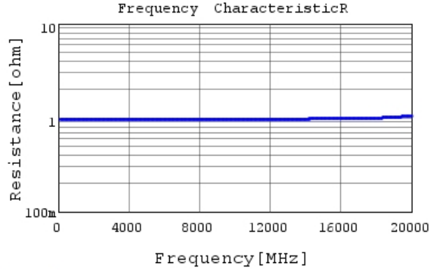
GRM0335C1HR20WA01 R DCOV, 25degC
