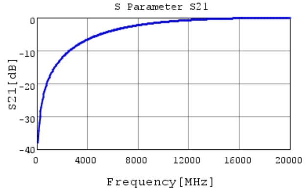
GRM0335C1HR20WA01 S21 DCOV, 25degC
