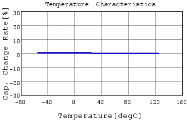
GRM0335C1HR20WA01 C-Temp. capchange, DCOV, 1
