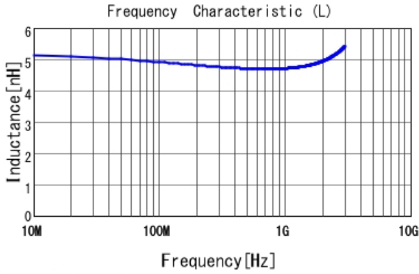
LQP03TN4N7HZ2 L
