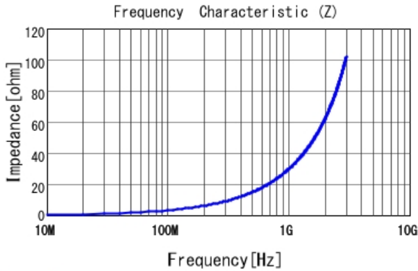
LQP03TN4N7HZ2 |Z|
