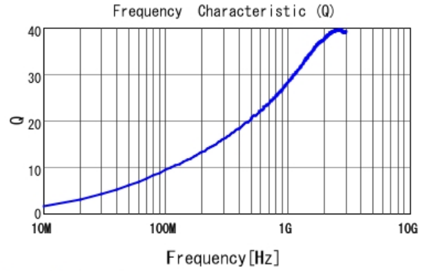
LQP03TN4N7HZ2 Q
