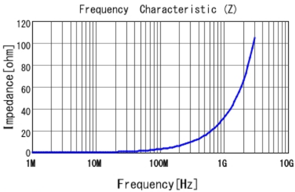
LQW15AN5N1C80 |Z|
