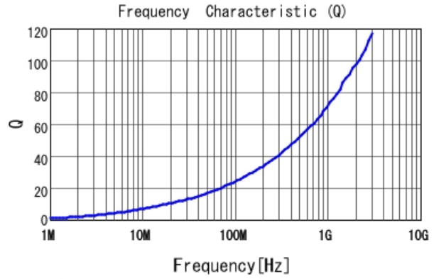
LQW15AN5N1C80 Q
