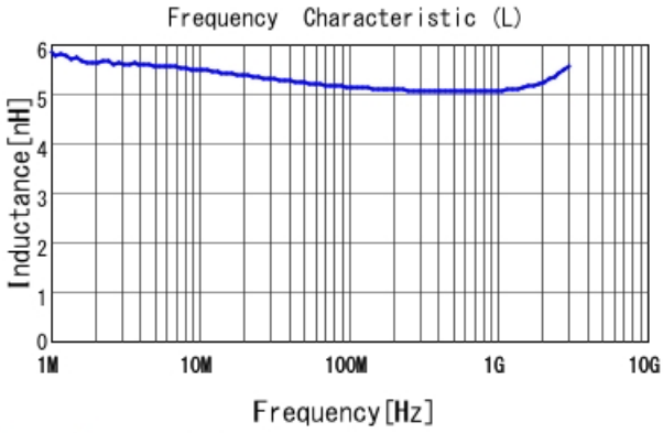
LQW15AN5N1C80 L
