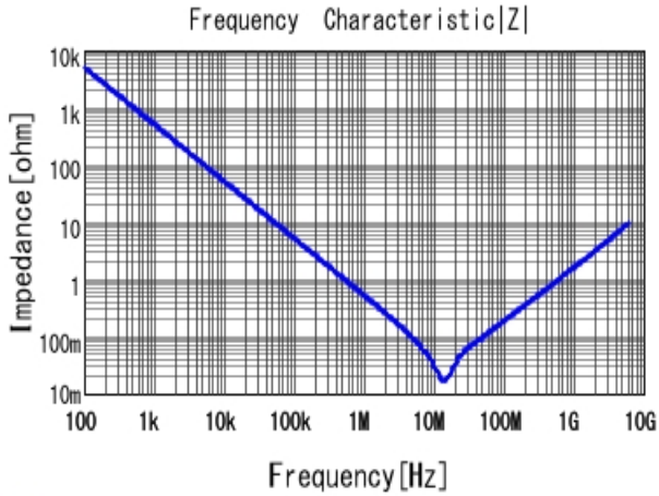
■ GRM155R60J334KE01 |Z| DCOV, 25degC
