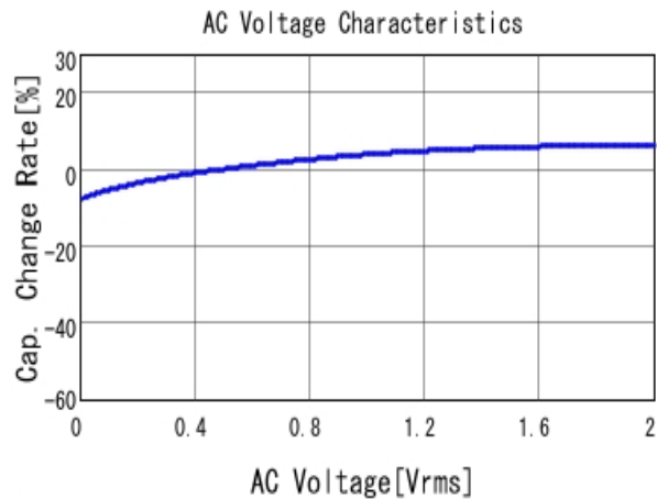
■ GRM155R60J334KE01 C-AC Voltage capchange, DCOV, 25.0d
