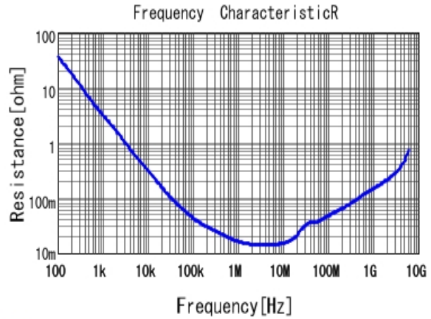
■ GRM155R60J334KE01 R DCOV, 25degC
