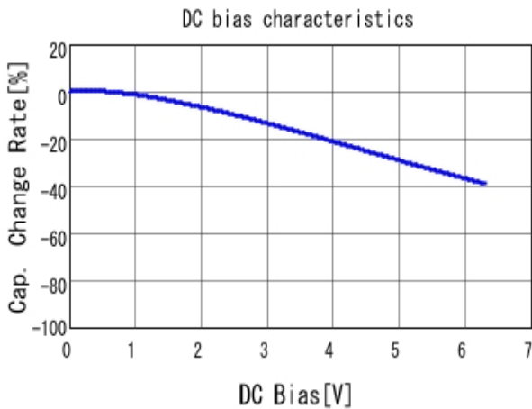
■ GRM155R60J334KE01 C-DC bias capchange, 25.0degC, AC0.
