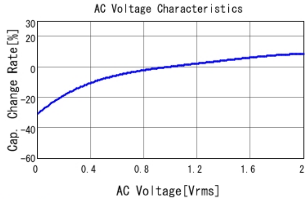
GRM21BR61E475KA12 C-AC Voltage capchange, DCOV, 25
