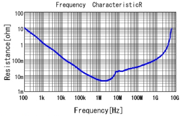
GRM21BR61E475KA12 R DCOV, 25degC
