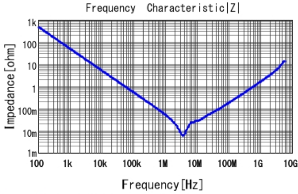
GRM21BR61E475KA12 |Z| DCOV, 25degC
