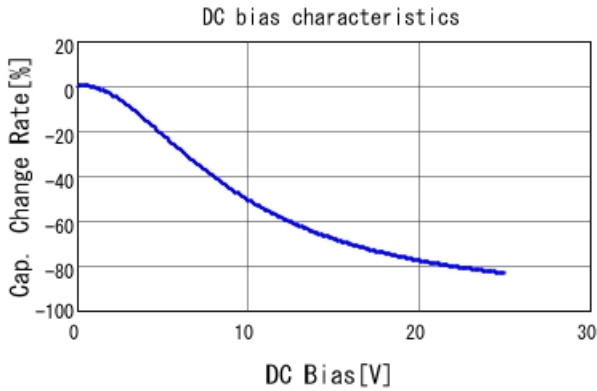
GRM21BR61E475KA12 C-DC bias capchange, 25.0degC, A
