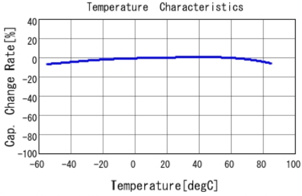
GRM21BR61E475KA12 C-Temp. capchange, DC0.0V, AC1.C
