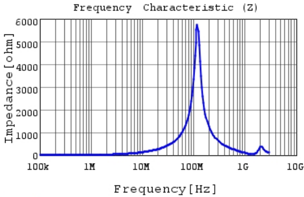
LQH32NZ2R2K23 |Z|
