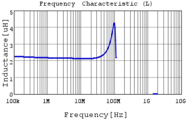
LQH32NZ2R2K23 L
