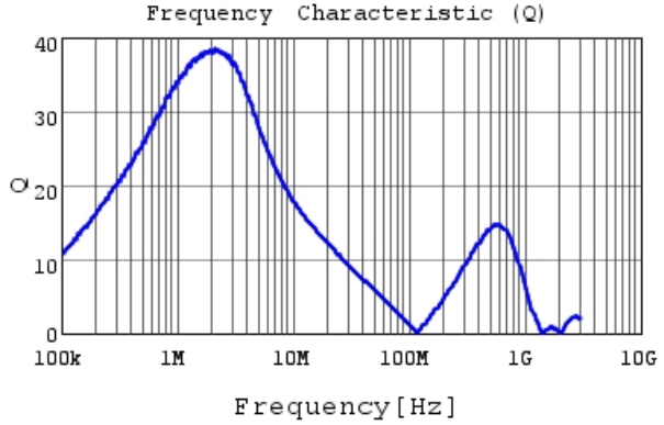
LQH32NZ2R2K23 Q
