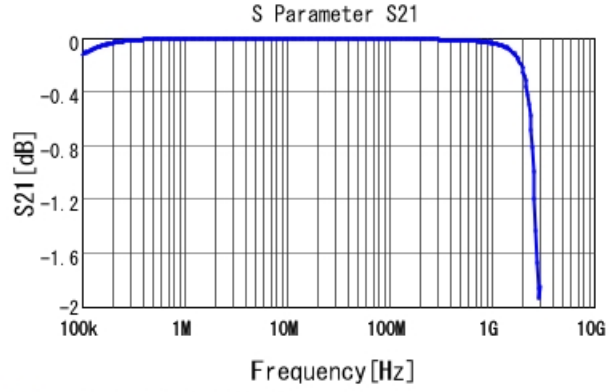
■ GA255DR7E2104MW01 S21 DCOV, 25degC
