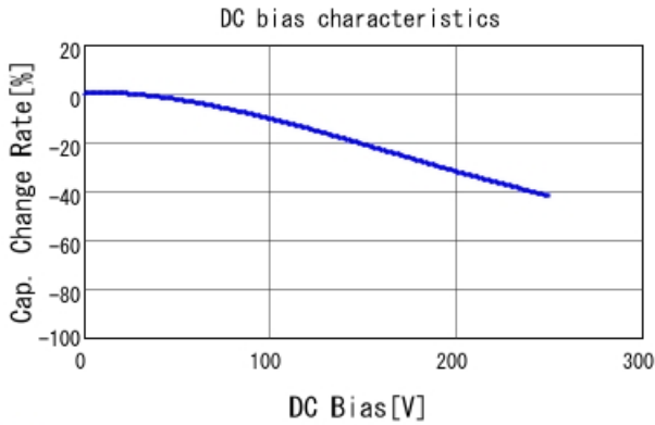
■ GA255DR7E2104MW01 C-DC bias capchange, 25.0degC, AC1V
