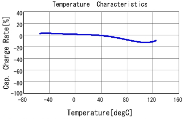
■ GA255DR7E2104MW01 C-Temp. capchange, DCOV, AC1Vrms
