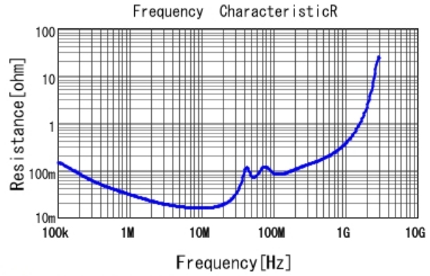
■ GA255DR7E2104MW01 R DC0V, 25degC
