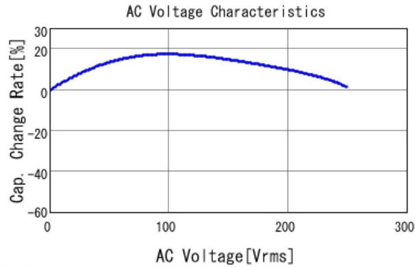
■ GA255DR7E2104MW01 C-AC Voltage capchange, DC0V, 25.0d
