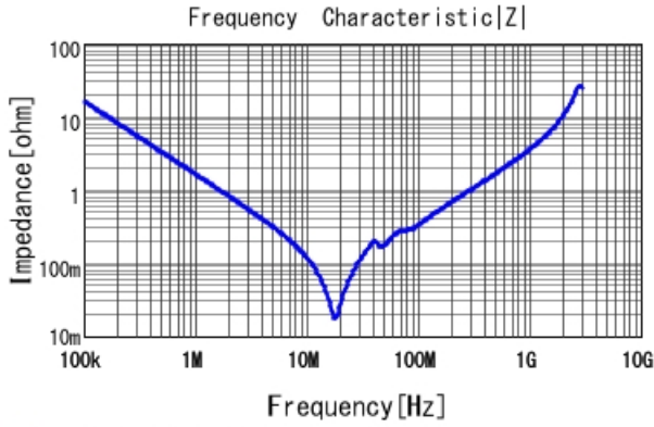
■ GA255DR7E2104MW01 |Z| DC0V, 25degC
