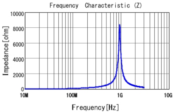
LQP03TNR13J02 |Z|
