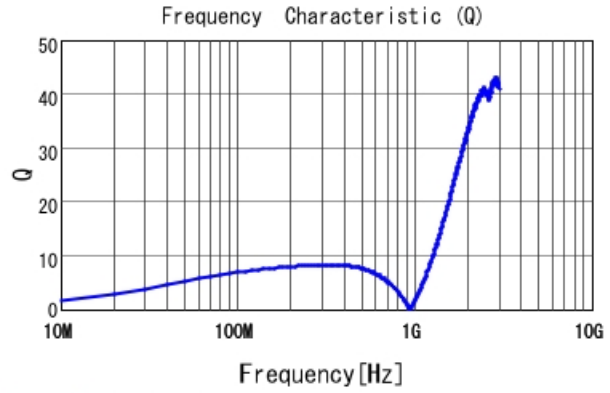
LQP03TNR13J02 Q
