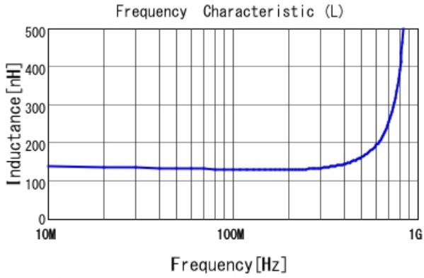
LQP03TNR13J02 L
