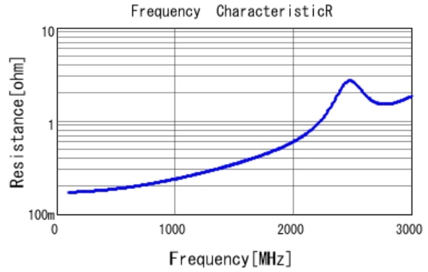
GRM21A5C2E330JW01 R DCOV, 25degC
