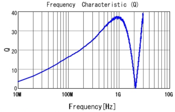
LQG15WZ43NG02 Q
