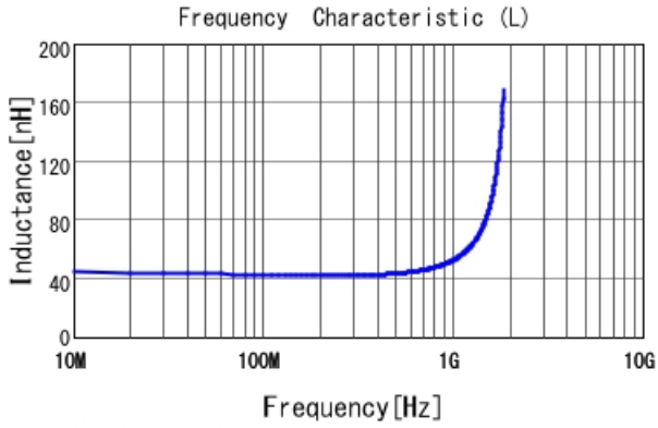
LQG15WZ43NG02 L
