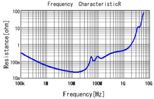
■ GRM43DR73A473KW01 R DCOV, 25degC
