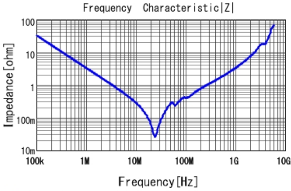
■ GRM43DR73A473KW01 |Z| DCOV, 25degC
