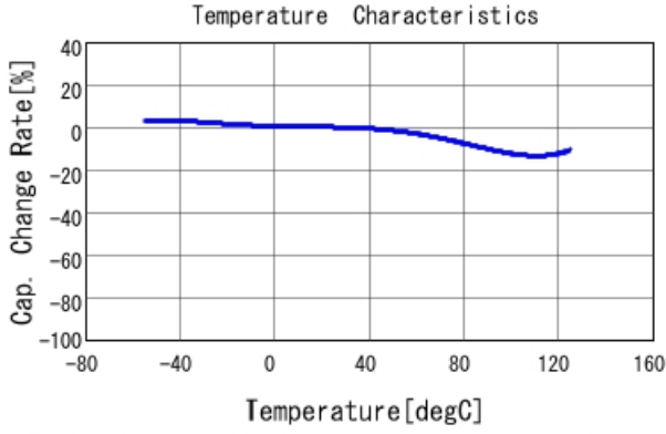
■ GRM43DR73A473KW01 C-Temp. capchange, DCOV, AC1Vrms
