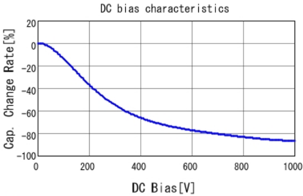
■ GRM43DR73A473KW01 C-DC bias capchange, 25.0degC, AC1V
