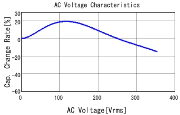
■ GRM43DR73A473KW01 C-AC Voltage capchange, DCOV, 25.0d
