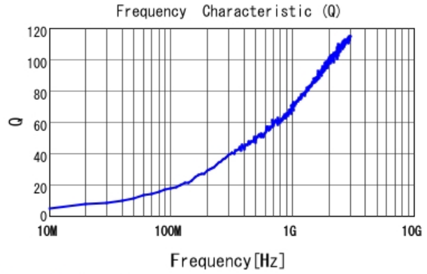
LQP03HQ1N0W02 Q
