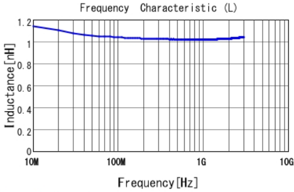
LQP03HQ1N0W02 L
