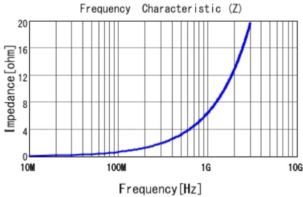
LQP03HQ1N0W02 |Z|
