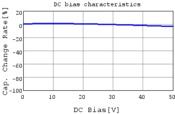
RDER71H471K0K1H03B C-DC bias capchange, 25.0
