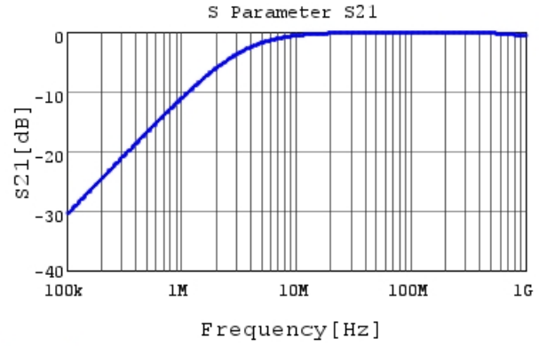
■ RDER71H471K0K1H03B S21 DC0V, 25degC
