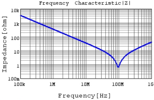
RDER71H471K0K1H03B |Z| DCOV, 25degC
