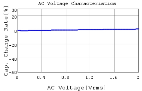
RDER71H471K0K1H03B C-AC Voltage capchange, I
