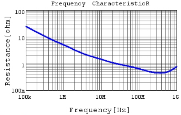
RDER71H471K0K1H03B R DCOV, 25degC
