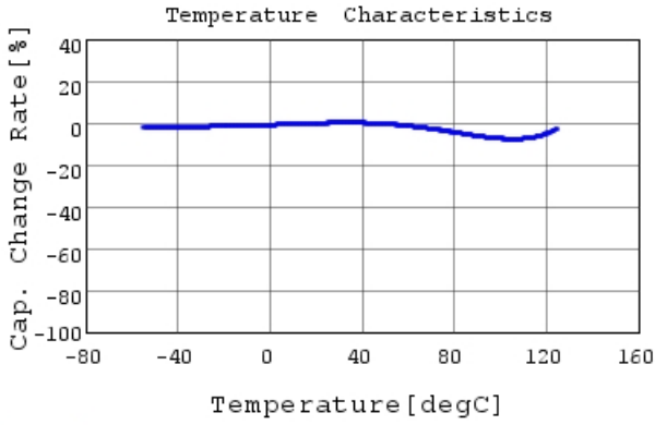
■ RDER71H471K0K1H03B C-Temp. capchange, DC0.0V
