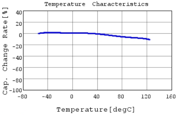
GCM155R71H473KE02 C-Temp. capchange, DC0.0V,
