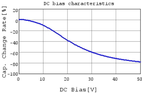
GCM155R71H473KE02 C-DC bias capchange, 25.0c
