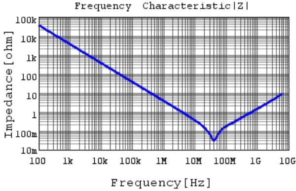
GCM155R71H473KE02 |Z| DC0V, 25degC
