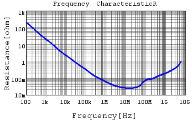
GCM155R71H473KE02 R DC0V, 25degC
