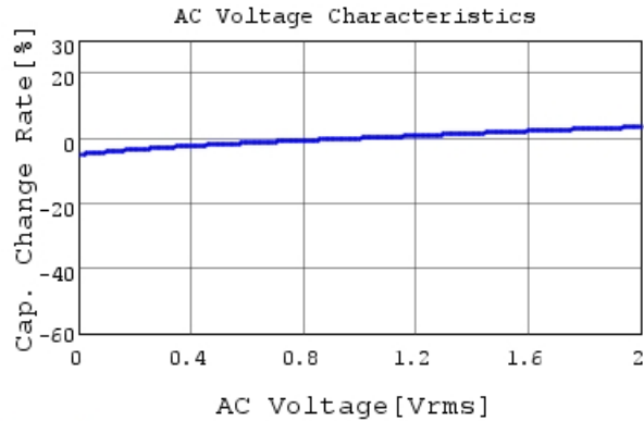
GCM155R71H473KE02 C-AC Voltage capchange, DC
