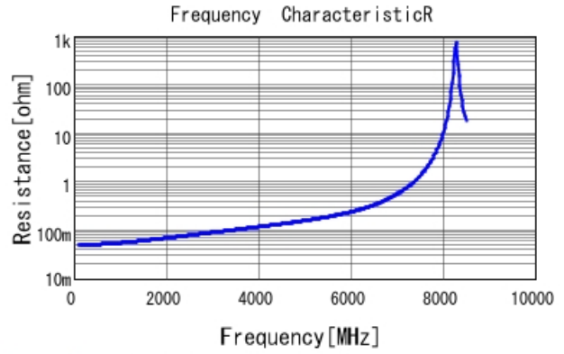
GQM2195C2E3R3BB12 R DCOV, 25degC
