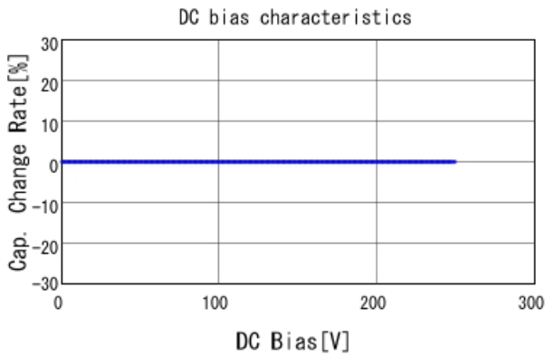
GQM2195C2E3R3BB12 C-DC bias capchange, 25.0degC, A
