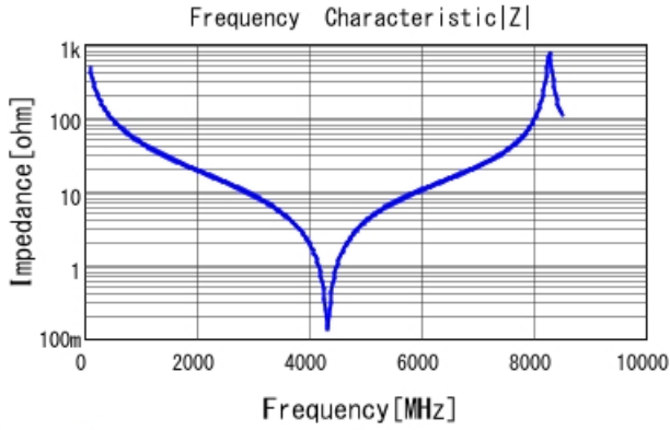
GQM2195C2E3R3BB12 |Z| DCOV, 25degC
