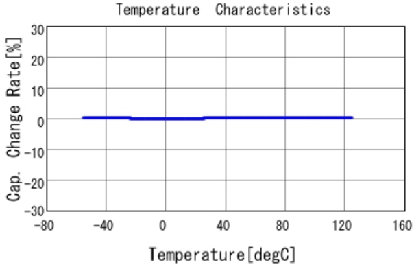
GQM2195C2E3R3BB12 C-Temp. capchange, DCOV, AC1Vrms
