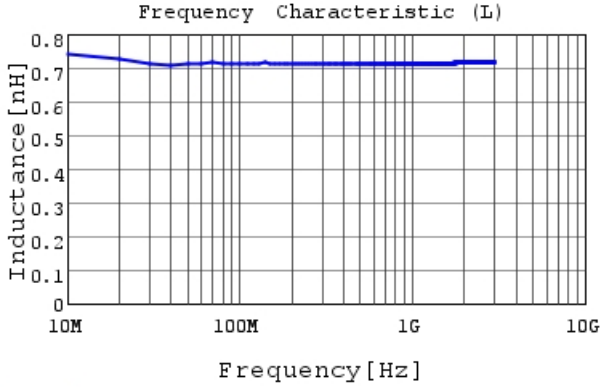
LQP03TQ0N7W02 L
