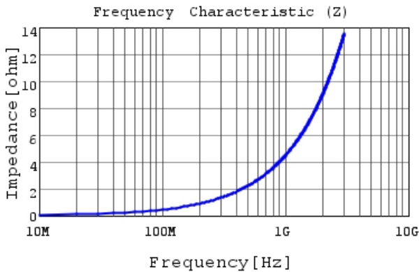
LQP03TQ0N7W02 |Z|
