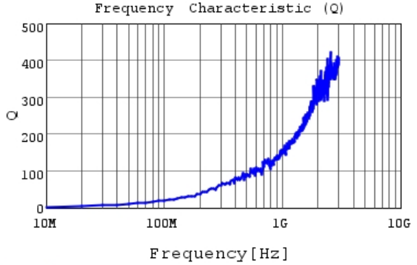
LQP03TQ0N7W02 Q
