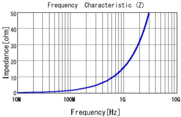
LQW15AN2N7D00 |Z|
