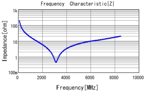
GRM1555C1H8R0CA01 |Z| DCOV, 25degC
