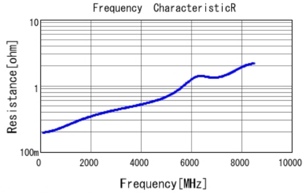
GRM1555C1H8R0CA01 R DCOV, 25degC
