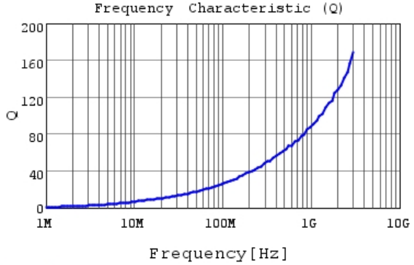
LQW15AN2N2C8Z Q
