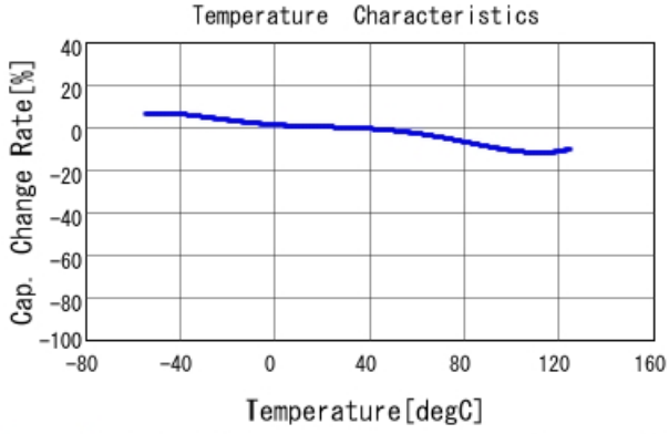
GRM21BR72E153KW03 C-Temp. capchange, DCOV, AC1Vrms
