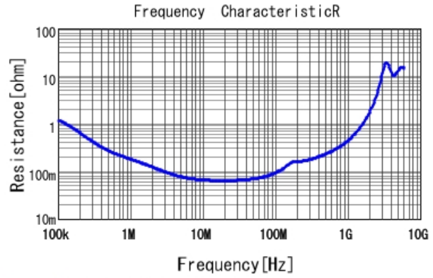
GRM21BR72E153KW03 R DCOV, 25degC
