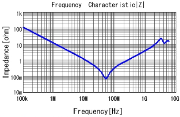
GRM21BR72E153KW03 |Z| DCOV, 25degC
