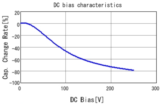
GRM21BR72E153KW03 C-DC bias capchange, 25.0degC, A
