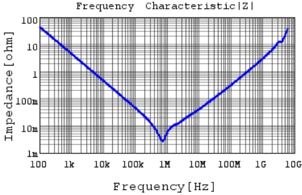
GRM31CE70J476ME15 |Z| DCOV,25degC
