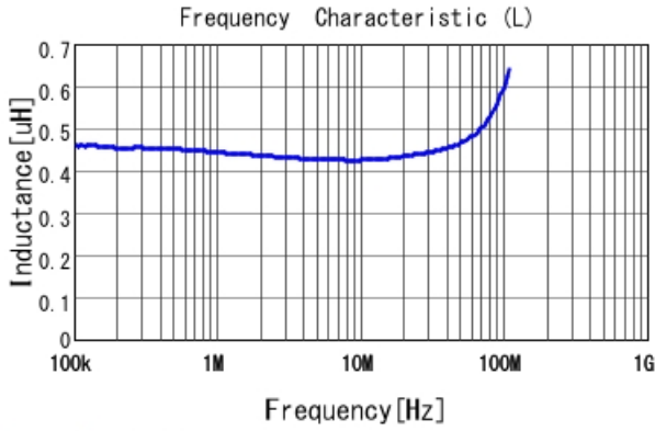
LQM2MPNR47NG0 L
