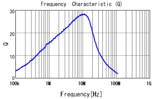
LQM2MPNR47NG0 Q
