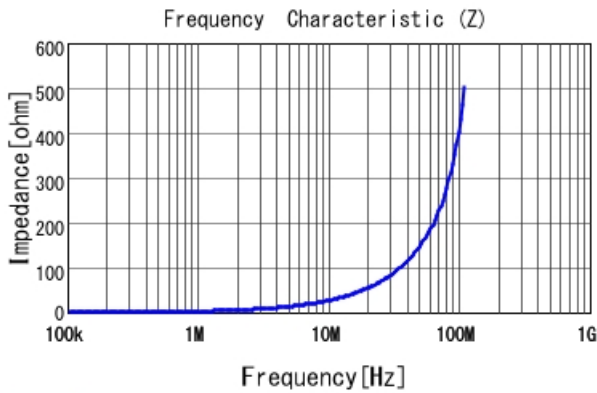
LQM2MPNR47NG0 |Z|
