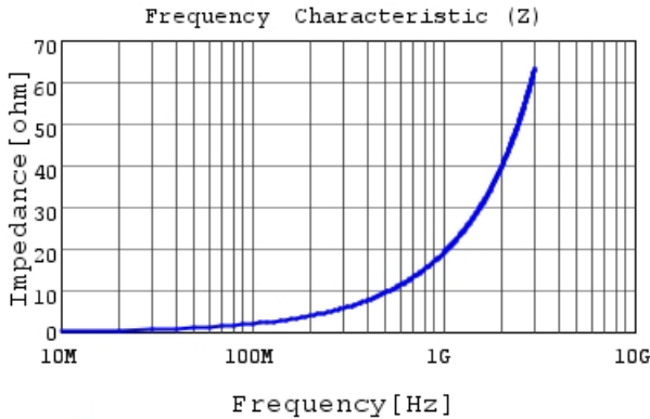
LQG15WH3N0S02 |Z|
