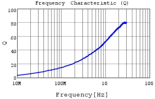
LQG15WH3N0S02 Q
