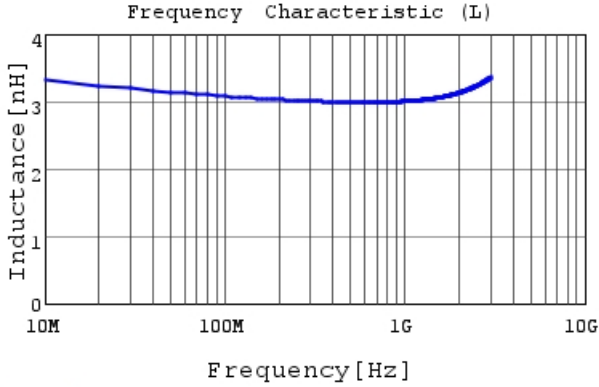
LQG15WH3N0S02 L
