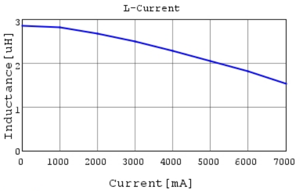
DFE322520FD-3R3M L-Current 20degC
