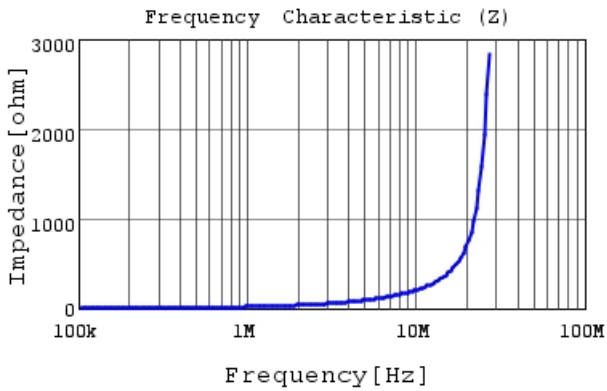
DFE322520FD-3R3M |Z|
