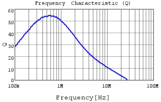
DFE322520FD-3R3M Q
