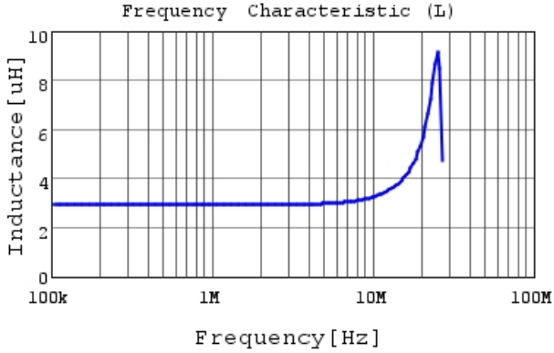
DFE322520FD-3R3M L
