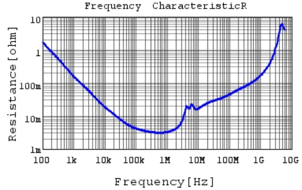
GCM31CC71H475KA03 R DC0V, 25degC
