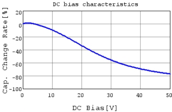
GCM31CC71H475KA03 C-DC bias capchange, 25.0c
