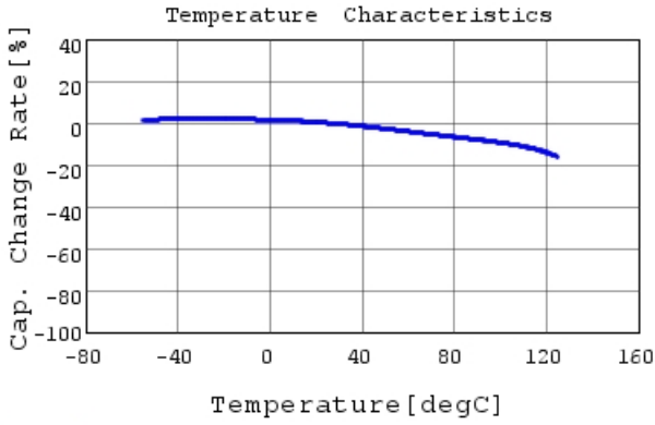
GCM31CC71H475KA03 C-Temp. capchange, DC0.0V,
