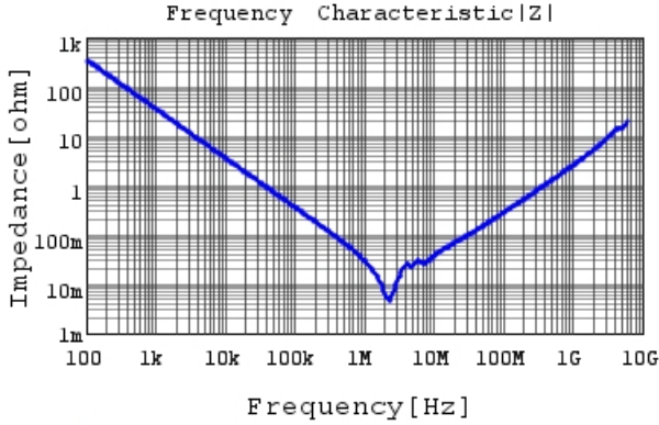
GCM31CC71H475KA03 |Z| DC0V, 25degC
