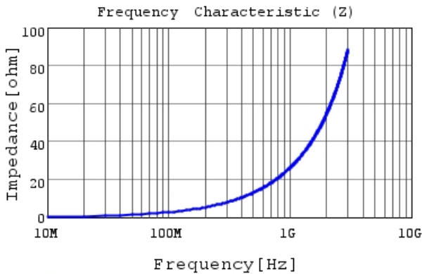
LQP03HQ4N1B02 |Z|
