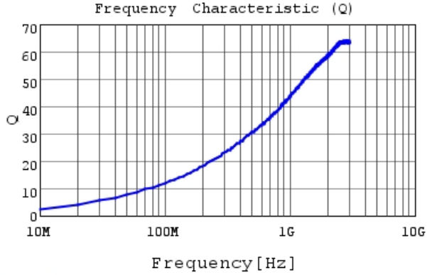
LQP03HQ4N1B02 Q
