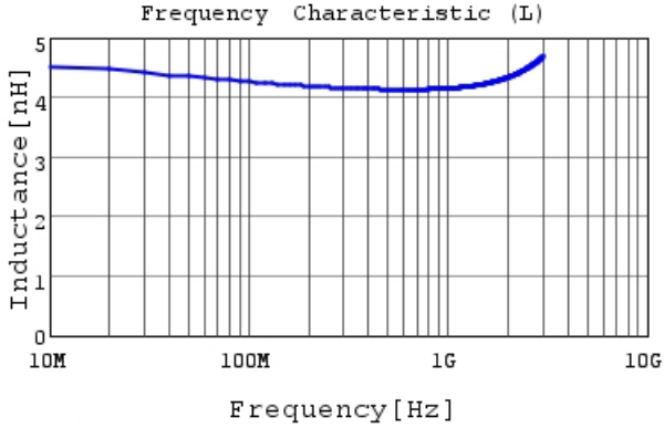
LQP03HQ4N1B02 L
