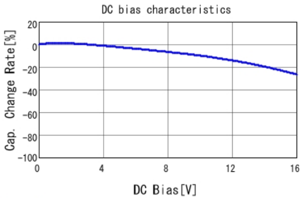
GCM188R71C104KA37 C-DC bias capchange, 25.0degC, A
