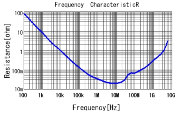
GCM188R71C104KA37 R DCOV, 25degC
