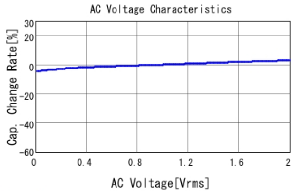
GCM188R71C104KA37 C-AC Voltage capchange, DCOV, 25
