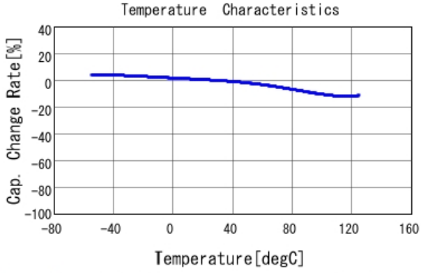
GCM188R71C104KA37 C-Temp. capchange, DC0.0V, AC1.C
