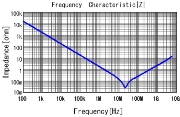
GCM188R71C104KA37 |Z| DCOV, 25degC
