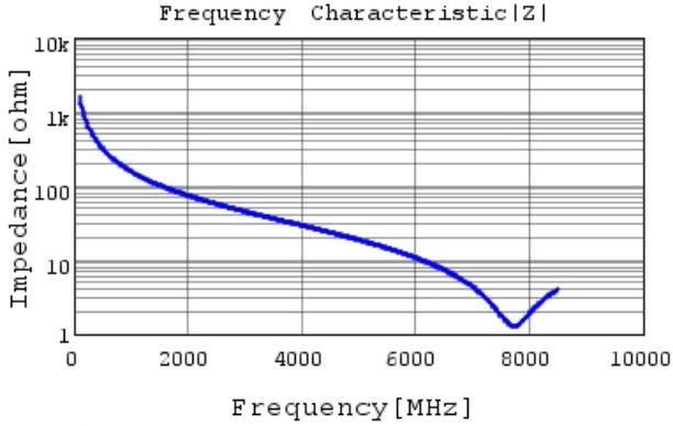
GCM1555C1H1R0BA16 |Z| DCOV, 25degC
