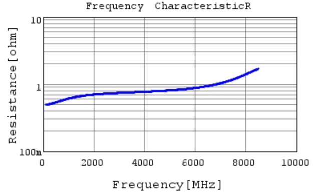
GCM1555C1H1R0BA16 R DCOV, 25degC
