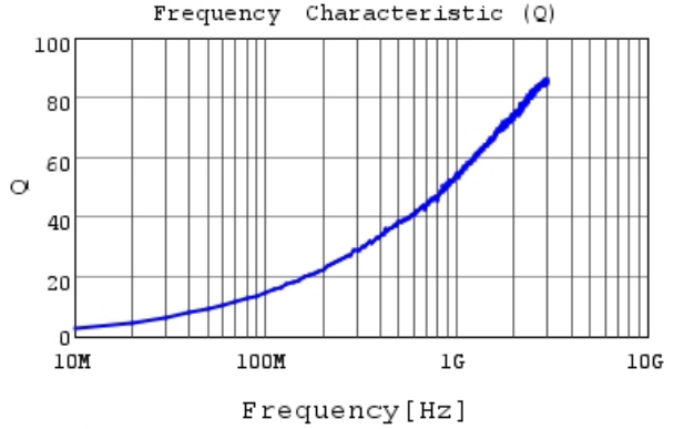
LQP03HQ1N8C02 Q
