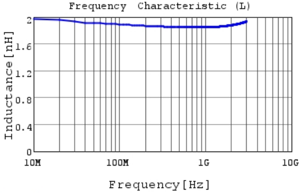
LQP03HQ1N8C02 L
