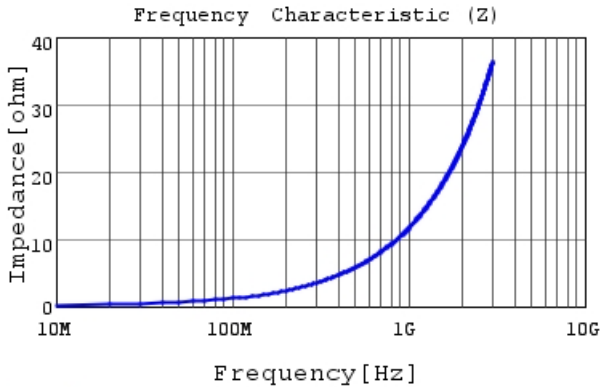
LQP03HQ1N8C02 |Z|
