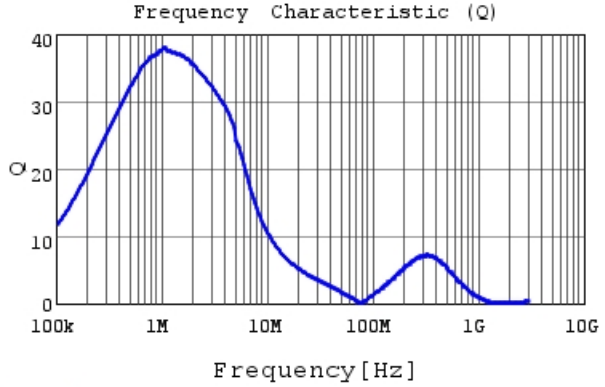
LQH3NPN2R2MGR Q
