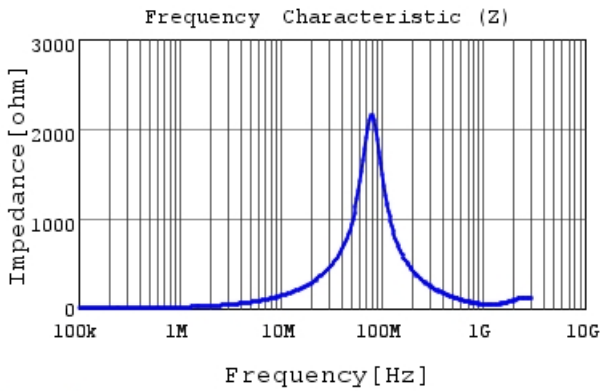
LQH3NPN2R2MGR |Z|
