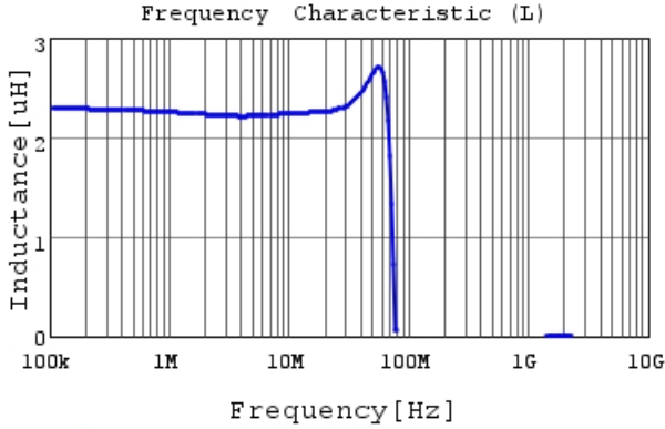
LQH3NPN2R2MGR L
