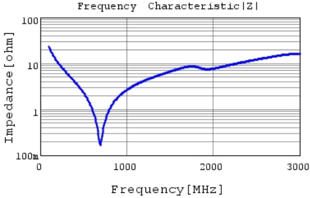
GRM31A7U3D680JW31 |Z| DC0V, 25degC
