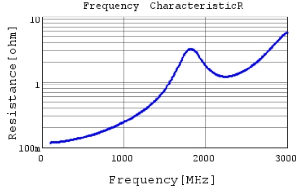
GRM31A7U3D680JW31 R DC0V, 25degC
