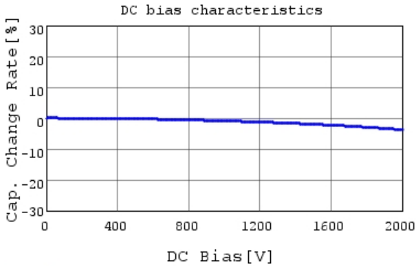
GRM31A7U3D680JW31 C-DC bias capchange, 25.0c
