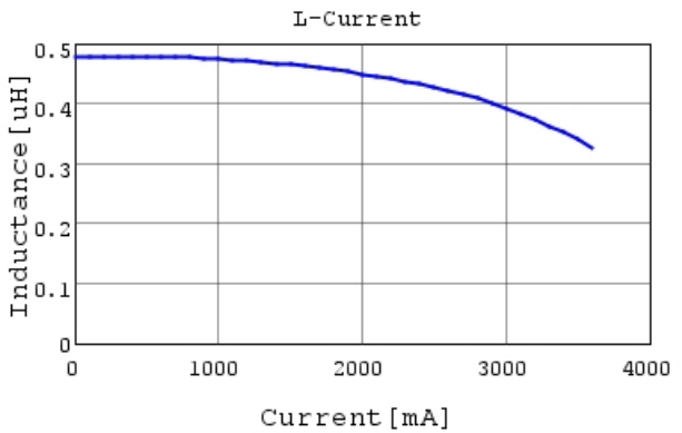
LQH2HPZR47NJR L-Current 20degC
