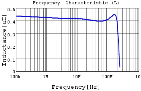
LQH2HPZR47NJR L
