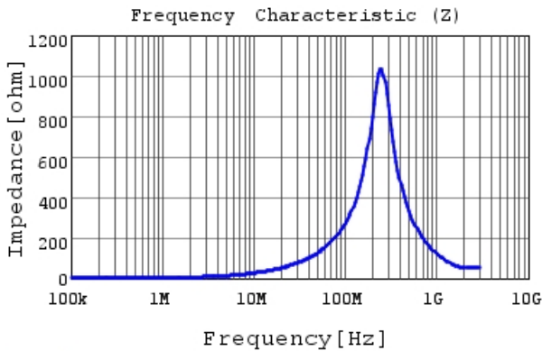
LQH2HPZR47NJR |Z|
