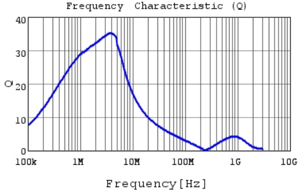
LQH2HPZR47NJR Q
