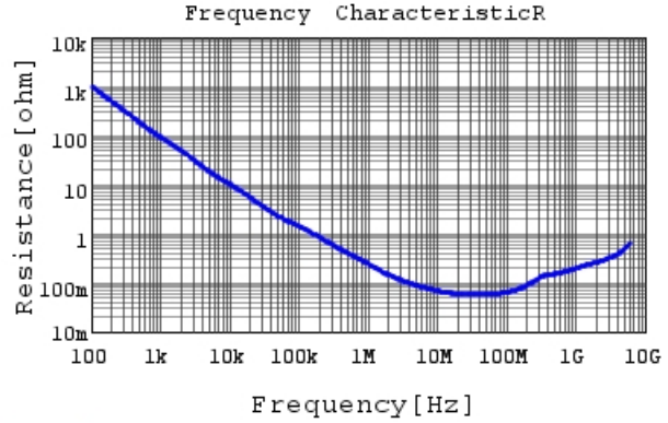
GRM033R70J103KA01 R DCOV, 25degC
