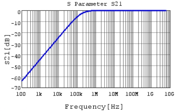
GRM033R70J103KA01 S21 DC0V, 25degC
