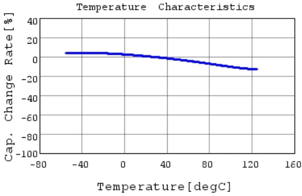
GRM033R70J103KA01 C-Temp. capchange, DC0.0V,
